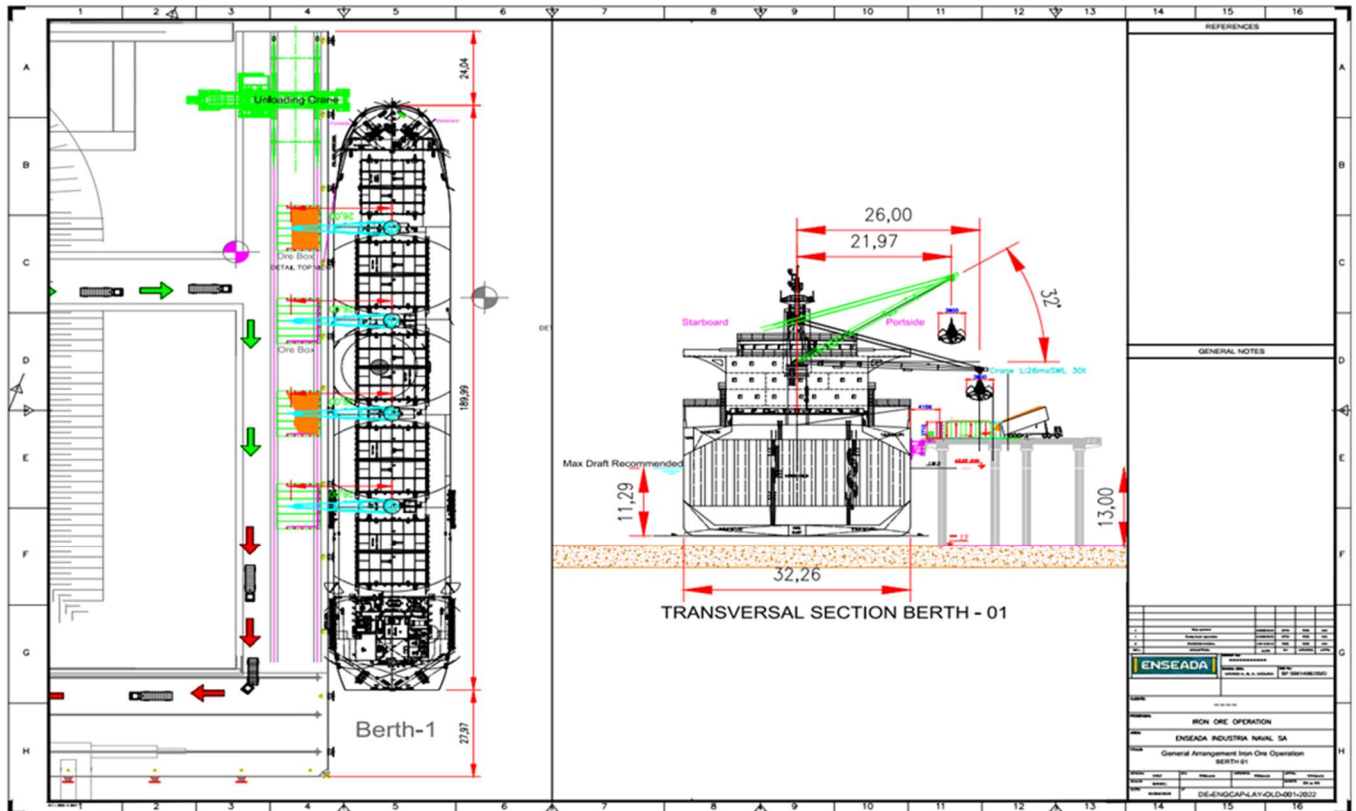
Figure 2 - General Arrangement of Berthing for Loading of grains Cargo in Bulk
